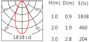
CMU1013 55° 4000K
