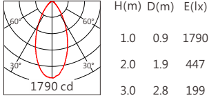
CMU1013 55° 3000K
