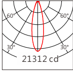
5050 30° RGBW(4000K)
