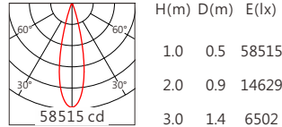
CMU1013 24° 4000K
