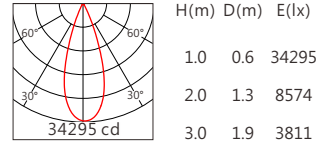
CMU1013 36° 4000K
