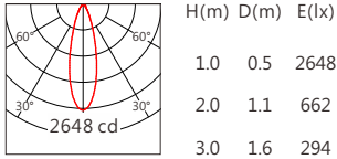
5050 30° RGBW(4000K)
