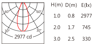
XP-L HI 45° 4000K
