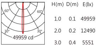
XP-L HI 30° 4000K
