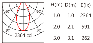
XP-L HI 55° 4000K
