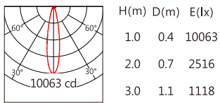
XP-L HI 20° 4000K
